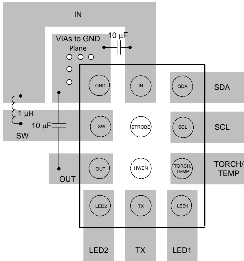
Figure 55. Layout Example
