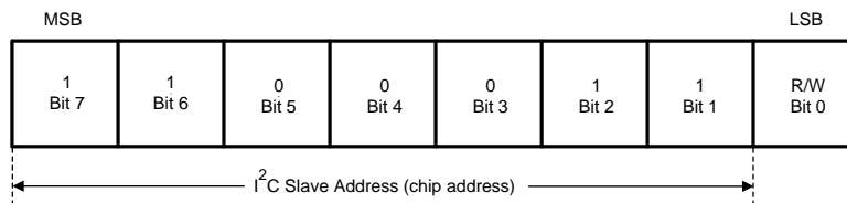
Figure 34. I 2 C-Compatible Chip Address
