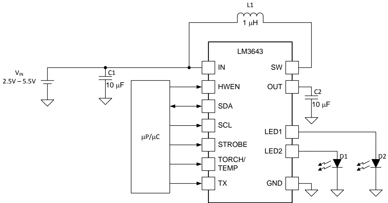
Figure 35. LM3643 Typical Application
